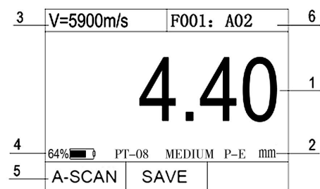
3.5 NORMAL MODE INTERFACE
