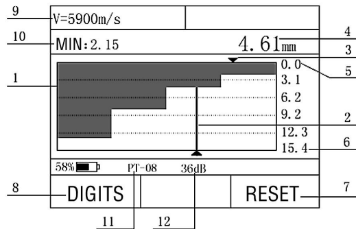
3.12 B scan interface diagram
