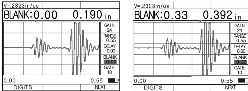
3.9 The waveform without blanking 3.10 omit the front noise waves by blanking
