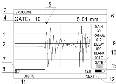
3.8 A-SCAN MODE INTERFACE
