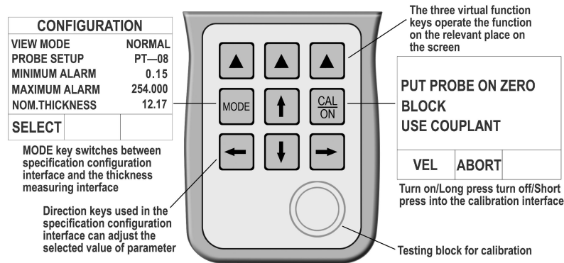
2.1 KEYBOARD FUNCTION ILLUSTRATION
