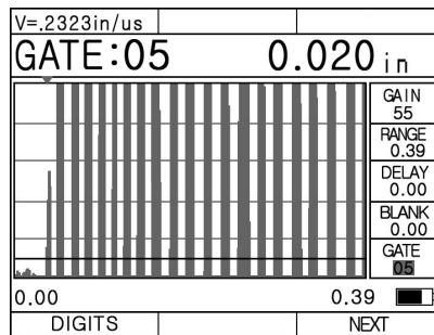
3.11 waveform of the 0.02in sheet by PT04
